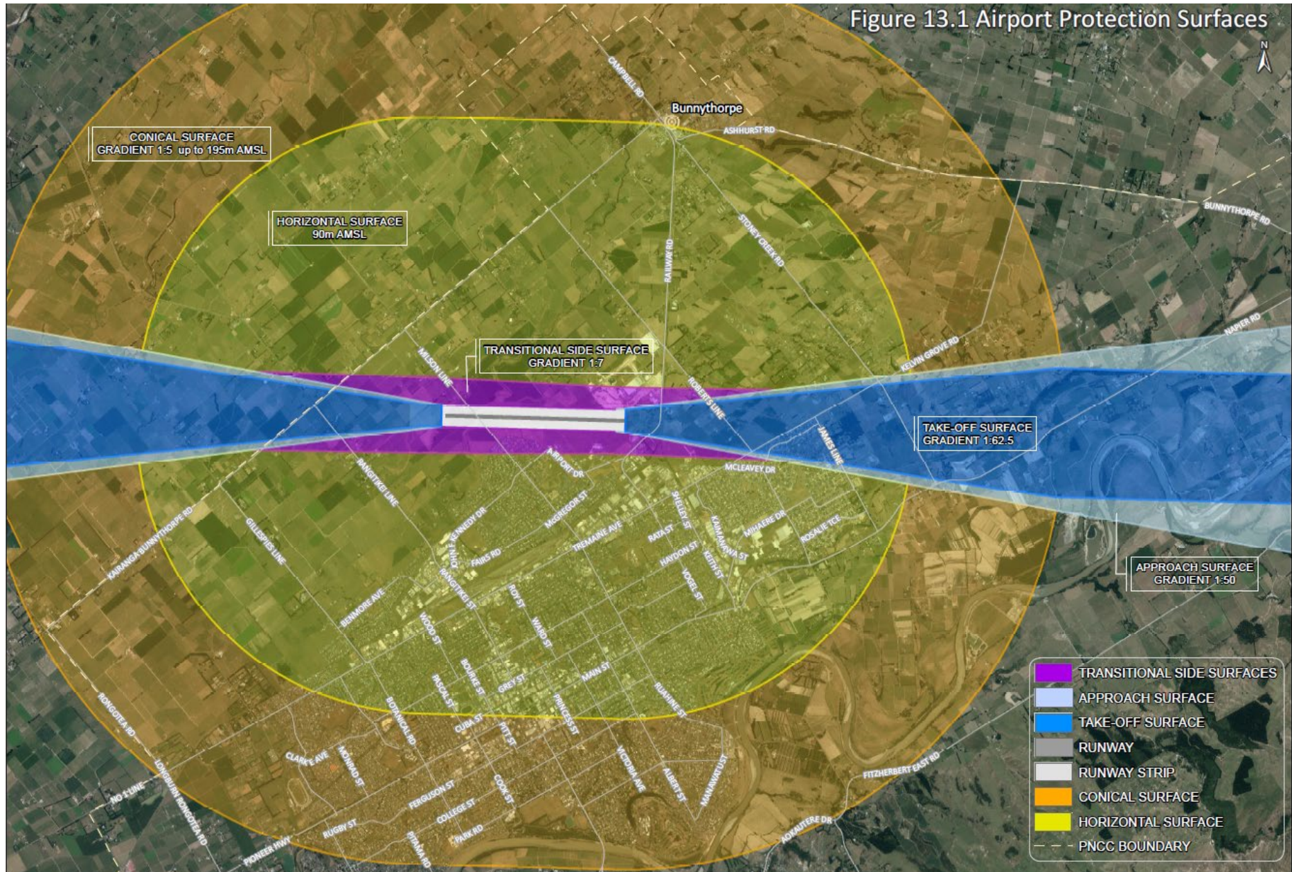
Figure 13.1 - Airport Protection Surfaces
